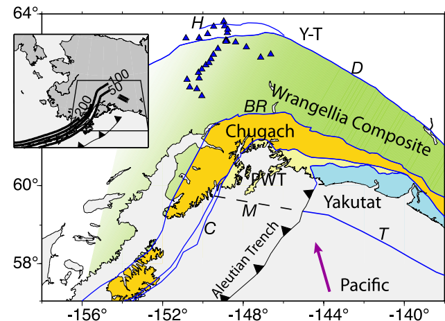
Figure 2. Southern Alaska composite terranes and bounding faults. Terrane abbreviations area PWT, Prince William Terrane; Y-T, Yukon-Tanana Terrane. Faults are BR, Border Ranges; C, Contact; D, Denali; H, Hines Creek; T, Transition. M, slope magnetic anomaly. Arrow shows direction of Pacific-North America motion, at 55 \text{ mm yr}^{-1} . Triangles denote BEAAR stations. From Plafker et al. [1994] and Brocher et al. [1994]. Inset shows area of map, and contours to slab at 50 km intervals labeled.
