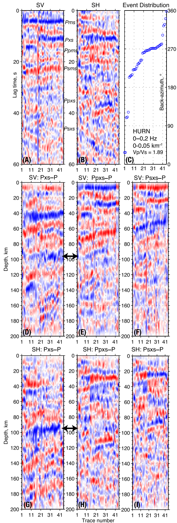
Figure 4. Sample data from station HURN, typical of well-sampled signals. (a) Deconvolved SV component for 46 events, sorted by back azimuth, low-pass filtered at 0.2 Hz. Blue shows positive-amplitude arrivals; red shows negative. Major predicted phases are labeled, for a nominal ray parameter ( 0.06 \text{ s km}^{-1} ), flat-lying interfaces, and provisional structure. (b) Deconvolved SH component. (c) Back azimuths to stations. (d)–(i) Results of moveout and sign correction, for SV (Figures 4d–4f) and SH (Figures 4g–4i). Traces are low-pass filtered below wave number of 0.05 \text{ km}^{-1} , and corrected so nominal sign of phase is positive (blue). Each trace applies moveout for a specific phase converting or reflecting off the slab Moho, as in Figure 1. Figures 4d and 4g are for Pxs ; Figures 4e and 4h are for Ppxs ; Figures 4f and 4i are for Psxs . Arrows show inferred slab Moho.
