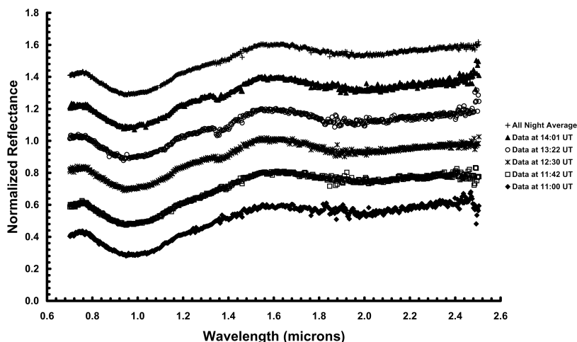
Fig. 6. Near-infrared spectra of (25143) Itokawa from the NASA IRTF taken on March 23, 2001 UT. Data are taken in groups and then averaged together to increase the signal-to-noise. One all-night average is also calculated and displayed here for comparison with the rest of the individual sets of spectra. All spectra are normalized and offset for clarity.
