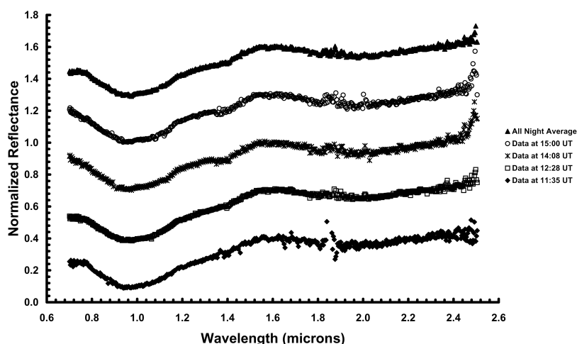
Fig. 7. Near-infrared spectra of (25143) Itokawa from the NASA IRTF taken on March 24, 2001 UT. Data are taken in groups and then averaged together to increase the signal-to-noise. One all-night average is also calculated and displayed here for comparison with the rest of the individual sets of spectra. All spectra are normalized and offset for clarity.
