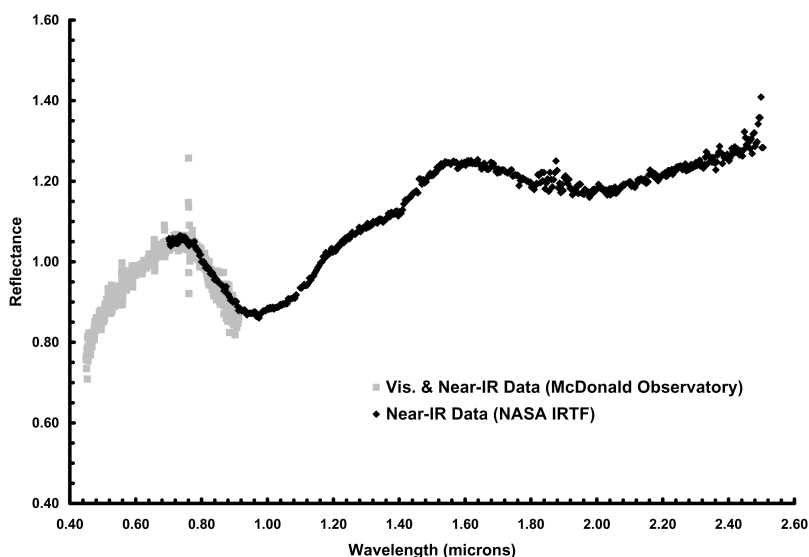
Fig. 8. The combined spectrum of visible and near-infrared data obtained of (25143) Itokawa on March 24, 2001 UT from McDonald Observatory and the NASA IRTF. Note the excellent agreement between the two datasets, particularly in the overlap region of the short wavelength wing of the 1.0 \mu m band.
