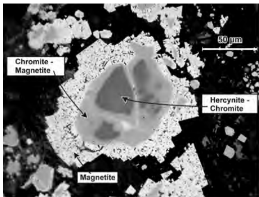
FIG. 7. Zoned spinel crystal from sample G2074 (reflected light, oil immersion). For compositions see Fig. 6.
