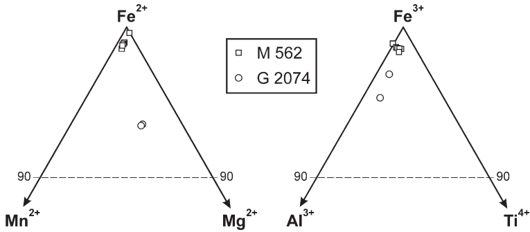
FIG. 4. Major substitutional deviations from end-member ferrous-ferric deerite, plotted as suggested by Vernié et al. (1986).
