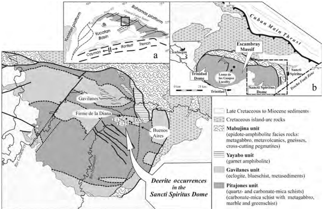
FIG. 1. Geological sketch map of the Escambray Massif indicating localities discussed in text.
