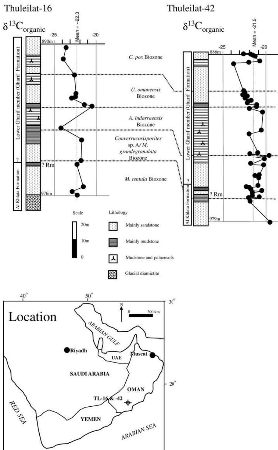
Fig. 2. Correlation of Thuleilat (TL) well sections of Oman based on palynology, and flattened on the base of the U. omanensis Biozone. Note that the boundaries between the Rahab member, the Al Khilata Formation and the Gharif Formation are not defined precisely in the Thuleilat wells. ? Rm, possible position of Rahab member. Reproduced with permission from Stephenson et al. (2005). Inset map shows location.
