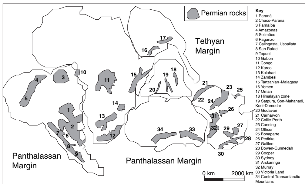
Fig. 1. Chief basins in the Early Permian of Gondwana.
