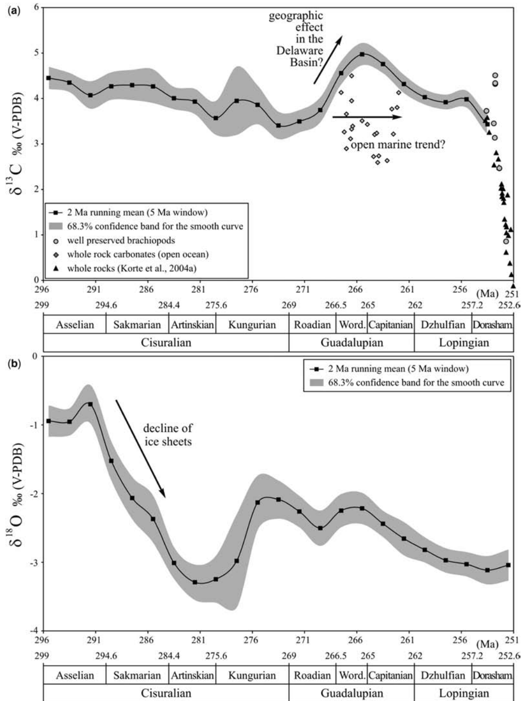
Fig. 4. Running \delta^{13}\text{C} mean (a) and \delta^{18}\text{O} mean (b) (2 Ma step, 5 Ma window), based on well-preserved brachiopod shells for the interval 296–253 Ma. The Early Permian brachiopod data are entirely derived from the Southern Urals, which were in a palaeo-equatorial position, although it is assumed that the brachiopods were living in basins which were open to the Tethys Ocean. Reproduced with permission from Korte et al. (2005).
